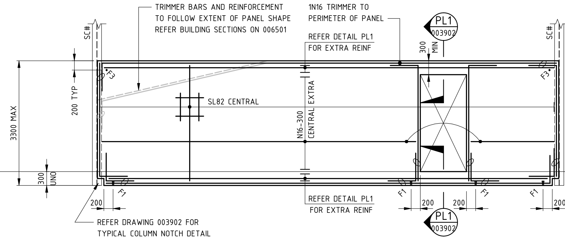
TYPICAL DADO PANEL TYPE - PW2 150 THICK PANEL
