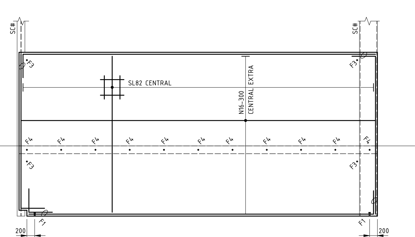
TYPICAL DADO PANEL TYPE - PW6 150 THICK PANEL
