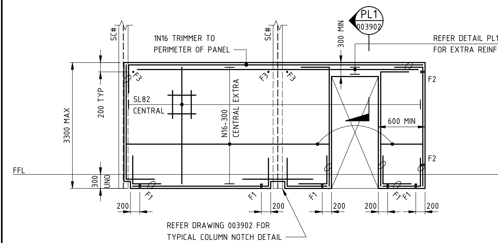
TYPICAL DADO PANEL TYPE - PW4 150 THICK PANEL
