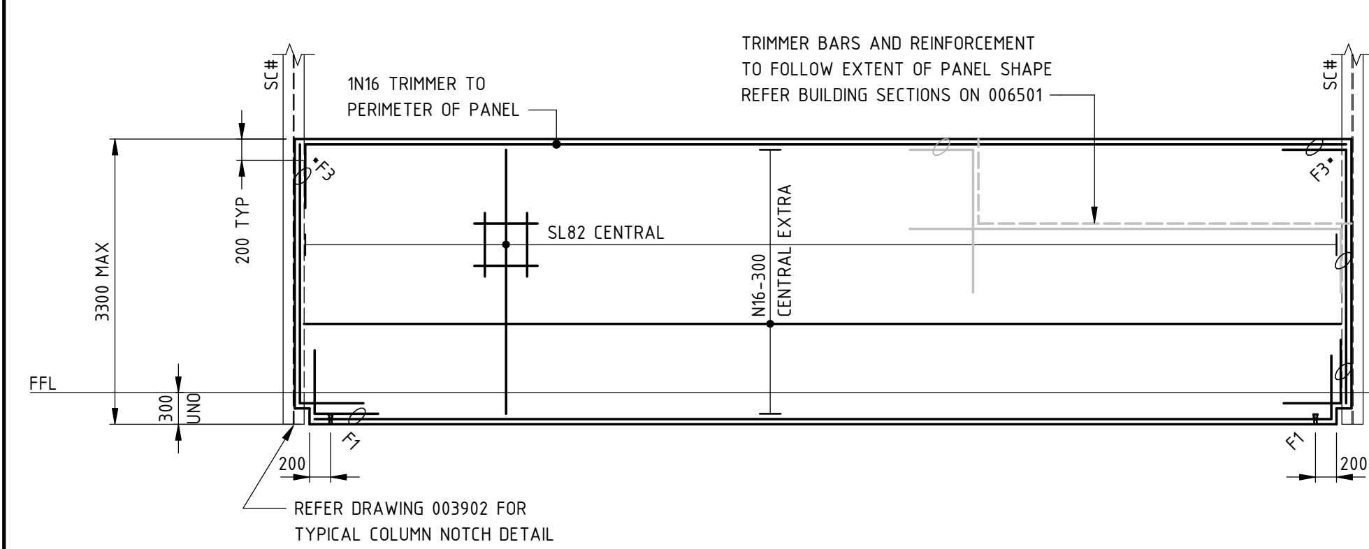
TYPICAL DADO PANEL TYPE - PW1 150 THICK PANEL
