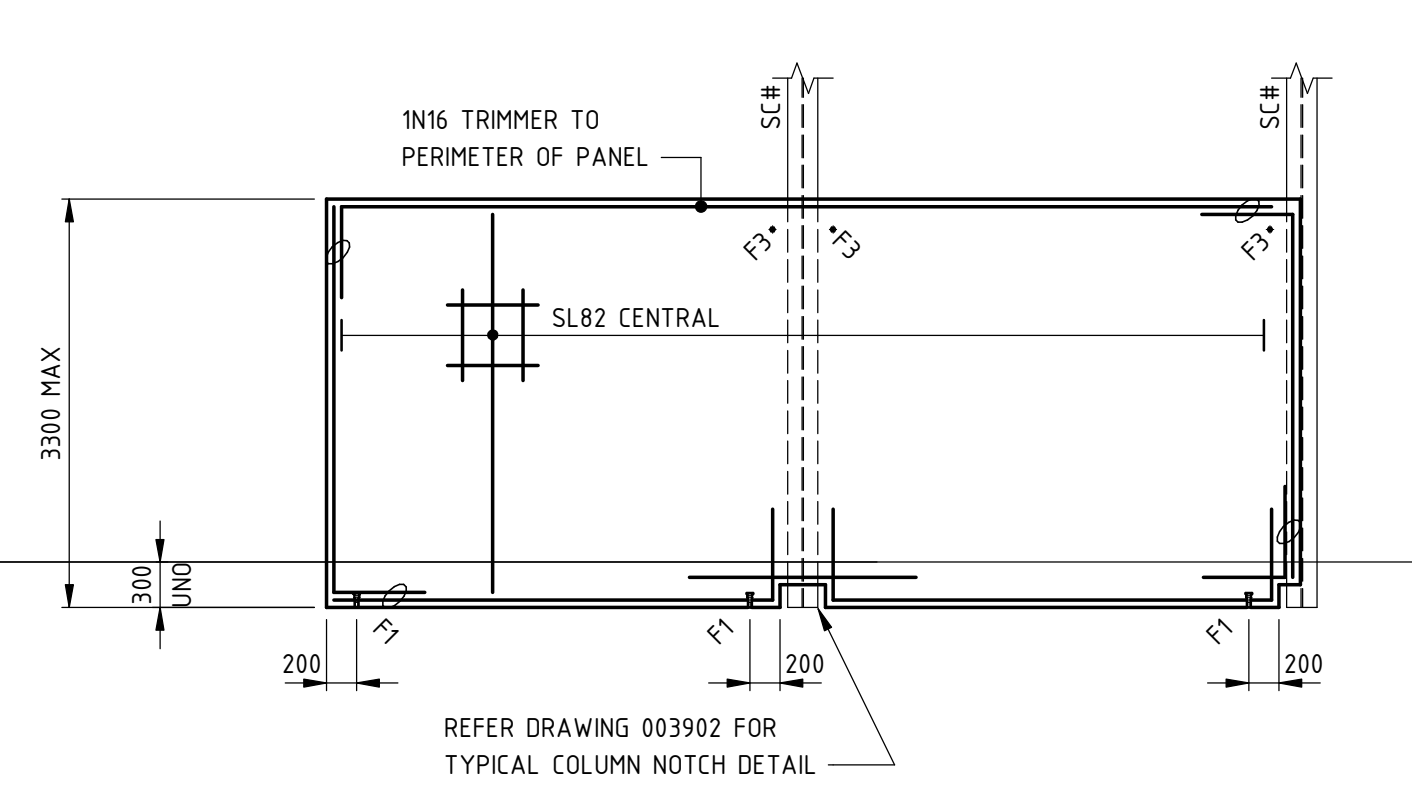
TYPICAL DADO PANEL TYPE - PW3 150 THICK PANEL
