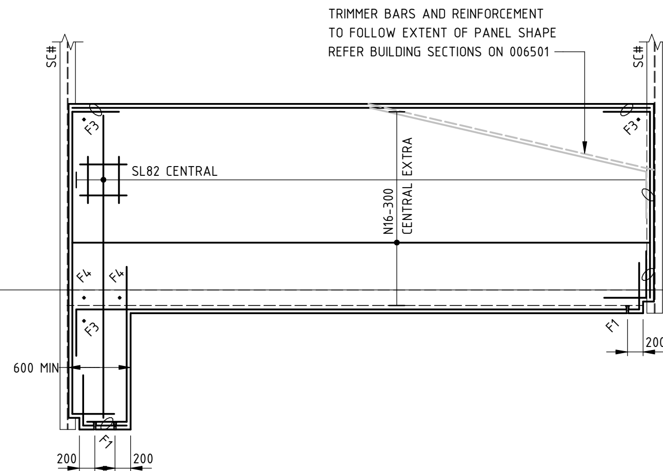
TYPICAL DADO PANEL TYPE - PW5 150 THICK PANEL
